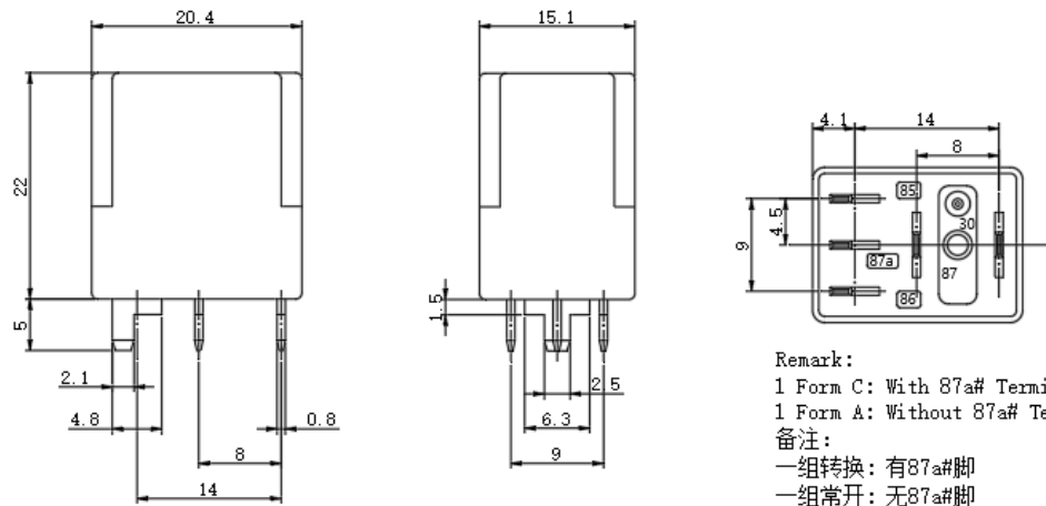
Wiring Diagram 接线图 (Bottom View 底部视图)
